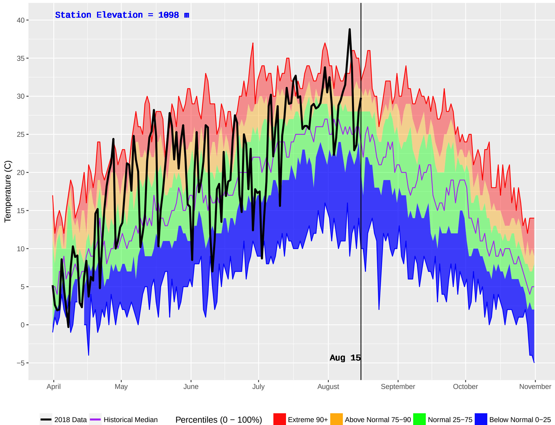
GOATFELL (401) : Historical (1986–2016) and Current (2018) Daily Temperature
