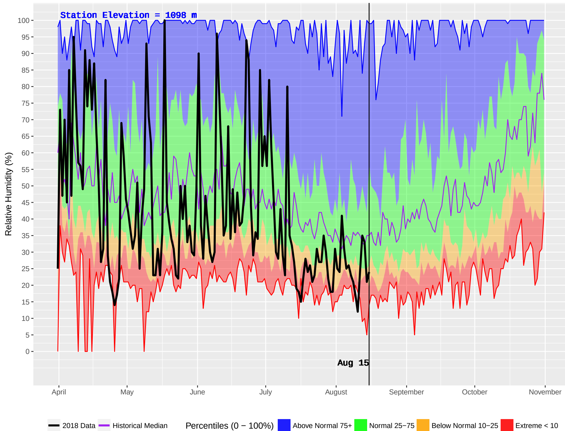
GOATFELL (401) : Historical (1986–2016) and Current (2018) Daily Relative Humidity
