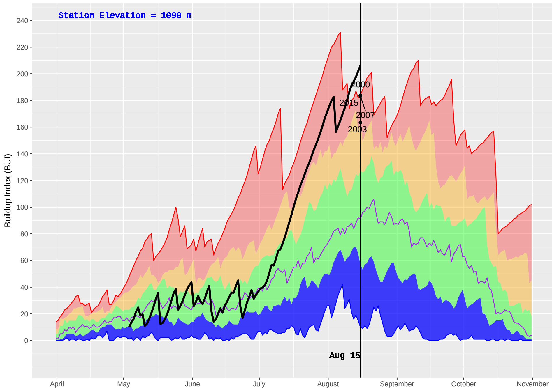
GOATFELL (401) : Historical (1986–2016) and Current (2018) Daily Buildup Index (BUI)
